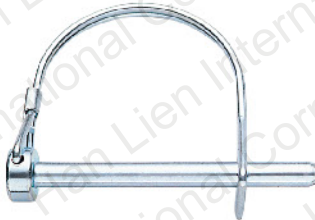
BP01-14234 Steel Wire Bail & Pin Bail Inside Width: 2" Bail Inside High: 1 13/16" Pin Size: 1/4" DIA. x 2 3/4" Available
