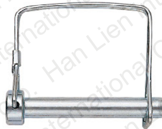
BP05-38212 Square Type Pin & Bail Square Inside Width: 2 1/8" Square Inside High: 1 11/16" Pin Size: 3/8" DIA. x 2 1/2" Available
