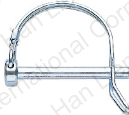
BP02-14 Steel Wire Bail & Pin (Tab-Lock) Bail Inside Width: 1 11/16" Bail Inside High: 1 11/16" Pin Size: 1/4" DIA. x 2 3/16" Available
