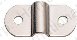
924S Sheet Steel Plate Hole Size: .172" Thickness: .039" Width: 1 1/16"
